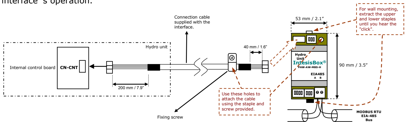
Figure 2.1 PAW-AW-MBS-H connection diagram
