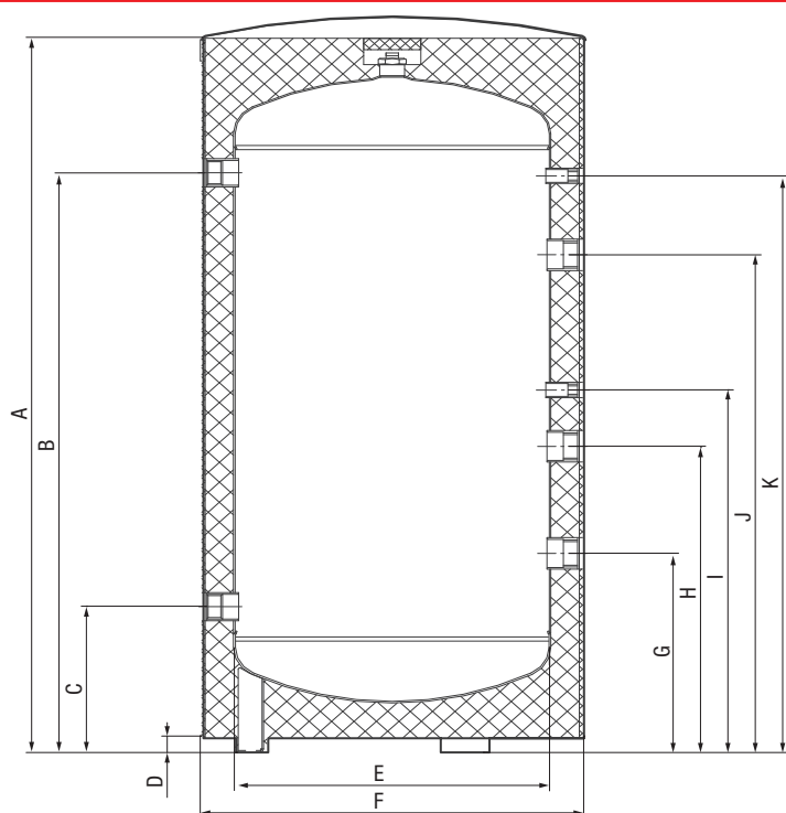
Pufferspeicher PS200-1/300-1/500-2
